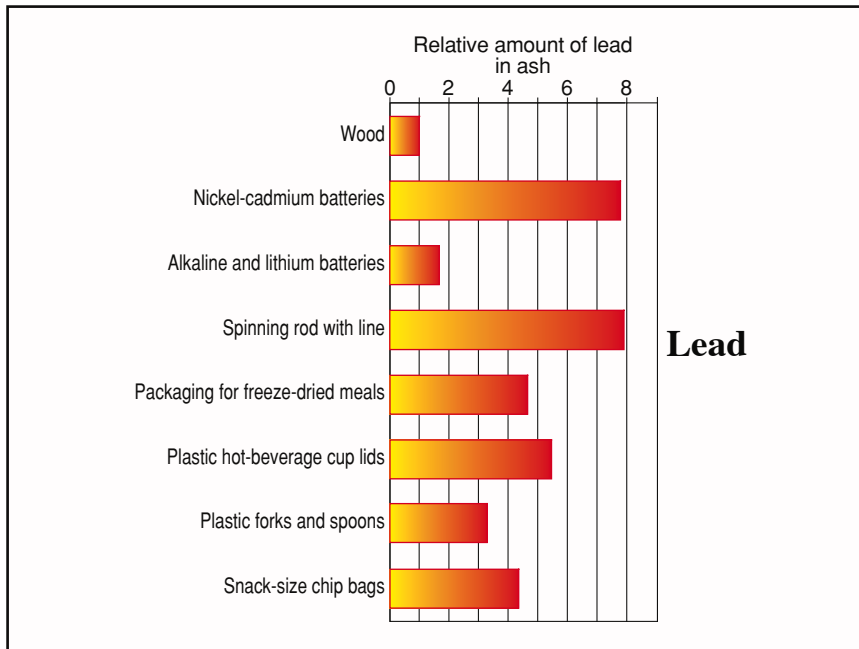
Figure 14—Some garbage items left elevated levels of lead—a suspected carcinogen—in the ash compared to a campfire that just burned wood.
